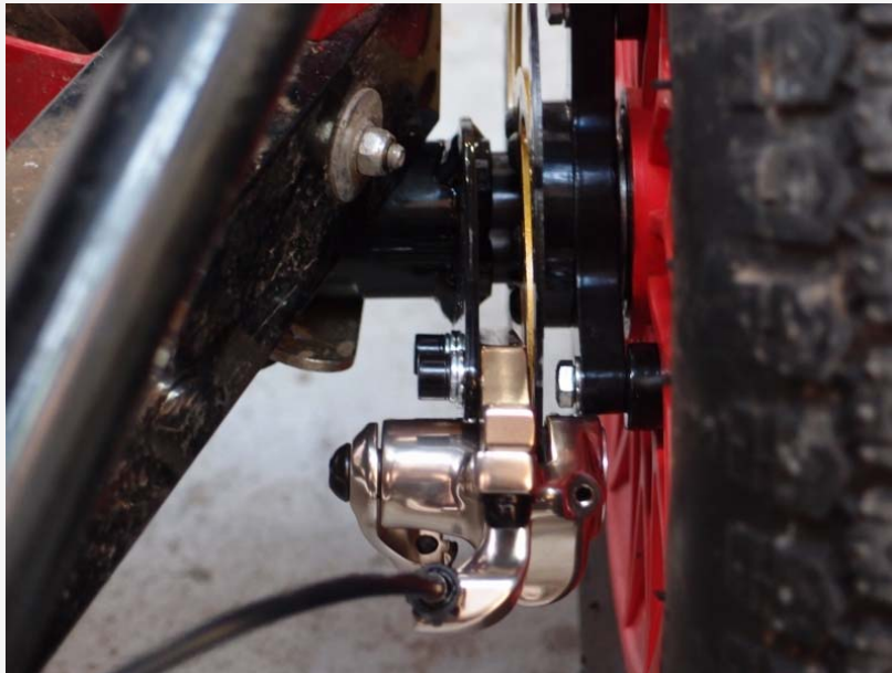
Disc brake caliper
