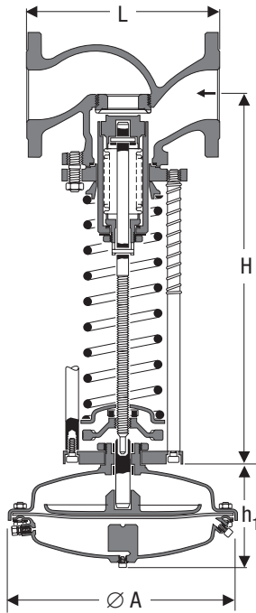
Pressure-reducing valve 5801
